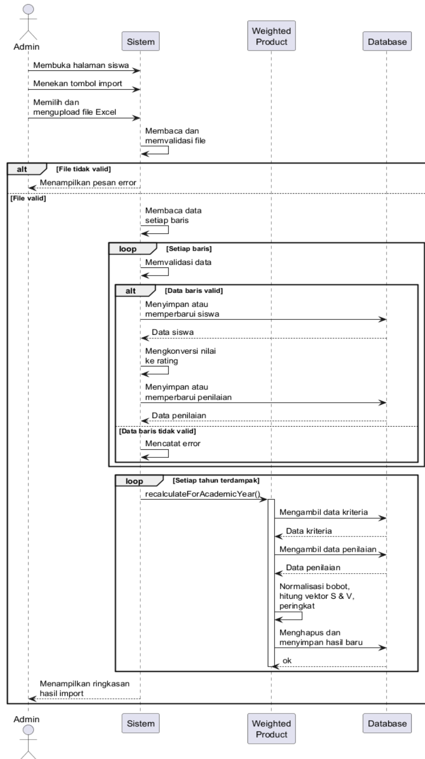
Gambar IV.16 Sequence Diagram Import Excel
