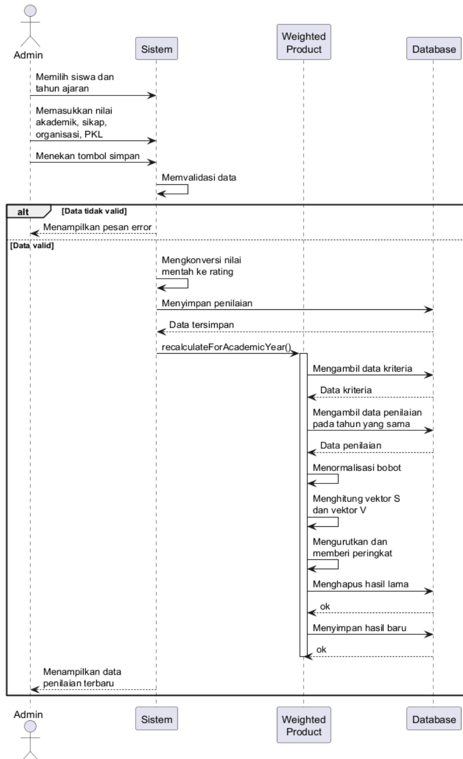
Gambar IV.15 Sequence Diagram Kelola Penilaian
