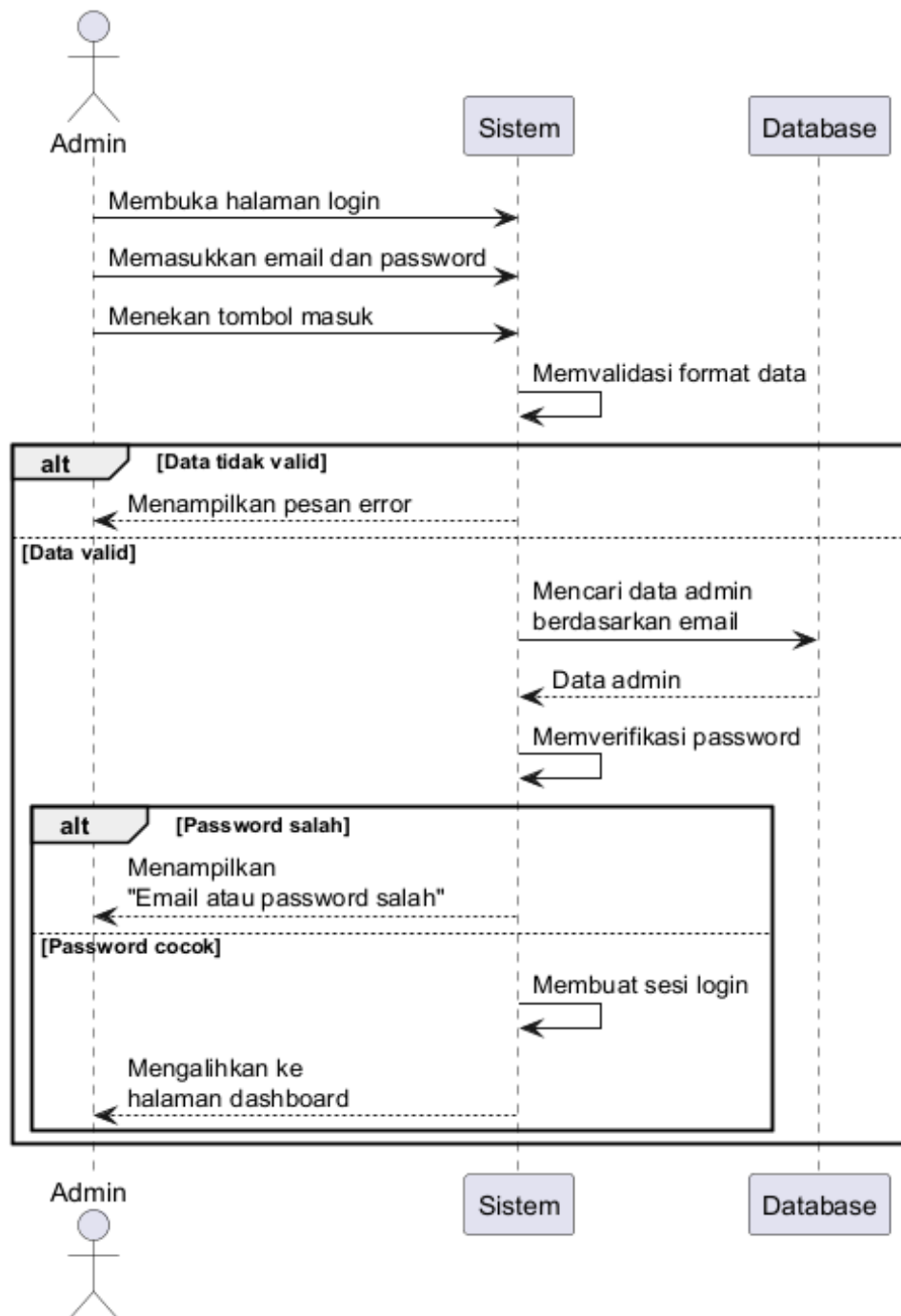
Gambar IV.14 Sequence Diagram Login
